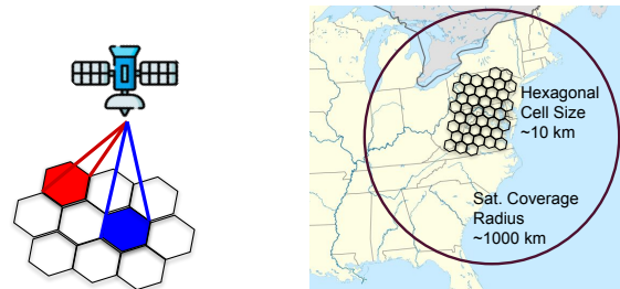
(a) A satellite can cover multiple cells using different beams. (b) The area of a cell is a small fraction of the total coverage area.
