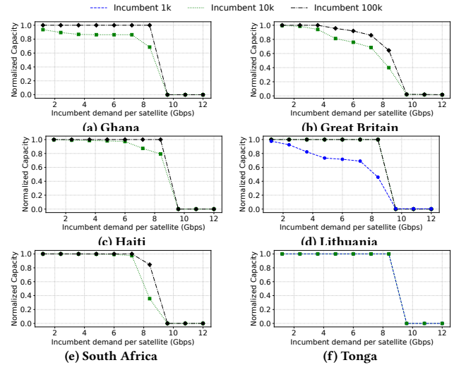
Figure 24: Estimated capacity for different incumbent demands per satellite.
