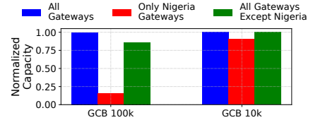
Figure 11: Ghana’s failover capacity with different gateway restrictions shows that reasonable data sovereignty constraints (e.g., All except Nigeria) do not impact capacity.
