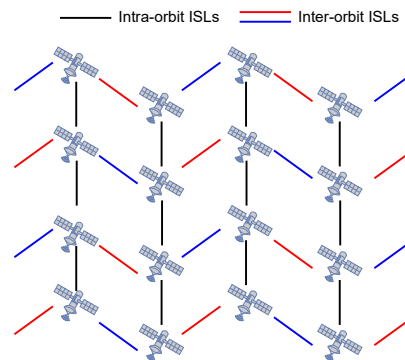
Figure 20: Depicting connectivity in a satellite network with three ISLs. With the +Grid connectivity, both the red and blue inter-orbit ISLs are used while for three ISLs, only the blue ones are used.
