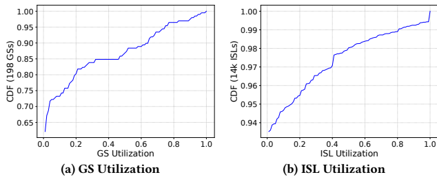
Figure 6: CDF of GS and ISL utilization for South Africa when 200k terminals with the GCB policy with no cap.
