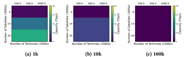
Figure 13: Impact of capped terminal distribution on South Africa’s estimated capacity with an expanding LEO network, highlighting how usable capacity quickly plateaus due to RF bottlenecks in densely populated areas.
