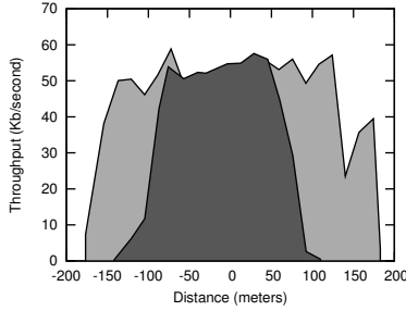
Figure 5. Throughput as a function of distance between two nodes in an urban environment. The light gray area shows LOS throughput, and the dark gray area shows ATC throughput. LOS and ATC conditions are described by Figure 6.
