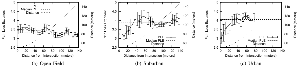
Figure 4. ATC measurements with median path loss exponents. Error bars show standard deviation of PLE.
