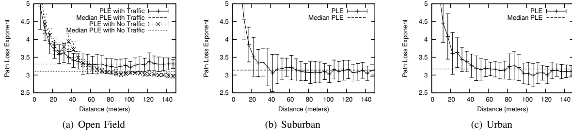
Figure 3. LOS measurements with median path loss exponents. Error bars show standard deviation of PLE. For the open field case, we show measurements with and without traffic.
