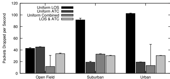
Figure 8. Median and 3rd quartile of packet drop rate.
