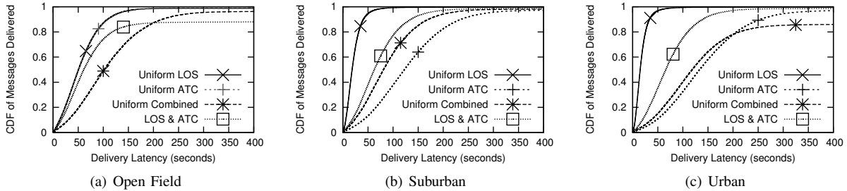
Figure 7. CDF of delivery latency for open-field, suburban and urban settings.
